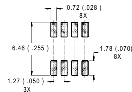
RECOMMENDED FOOTPRINT
