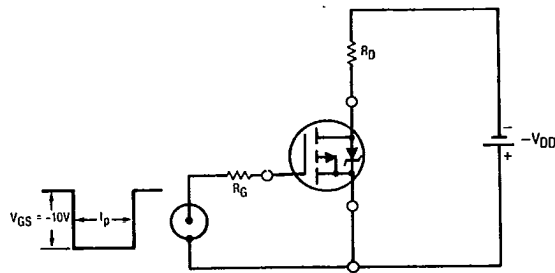
Fig. 15a — Switching Time Test Circuit
