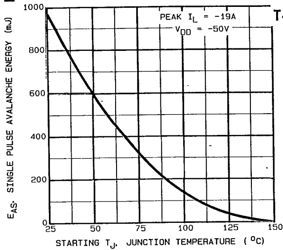
Fig. 14c — Maximum Avalanche Vs. Starting Junction Temperature
