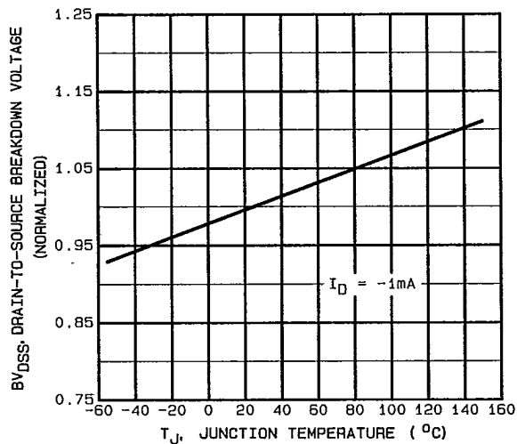
Fig. 8 — Breakdown Voltage Vs. Temperature
