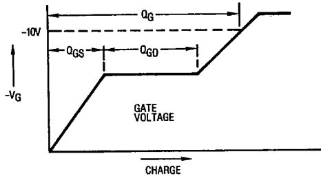
Fig. 16a — Basic Gate Charge Waveform
