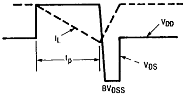
Fig. 14b — Unclamped Inductive Waveforms
