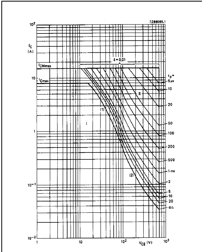
Fig.10. Forward bias safe operating area. T_{hs} < 25^\circ\text{C} (1) P_{tot max} line. (2) Second-breakdown limits (independent of temperature). I Region of permissible DC operation. II Permissible extension for repetitive pulse operation.
