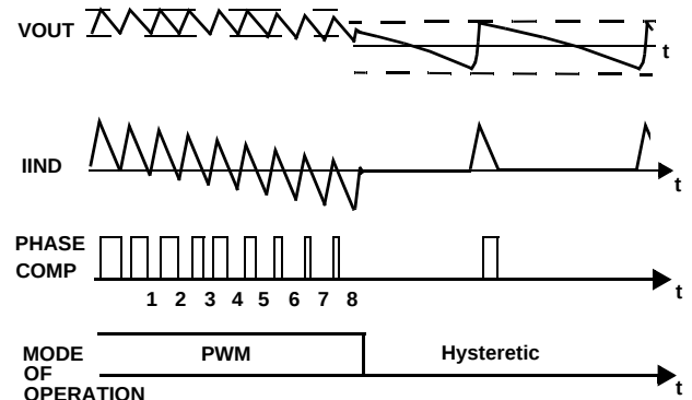
FIGURE 3. CCM -- HYSTERETIC TRANSITION
