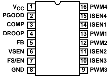
ISL6558 (16 LEAD SOIC) TOP VIEW
