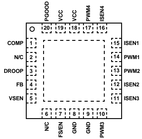
ISL6558 (20 LEAD 5X5 QFN) TOP VIEW
