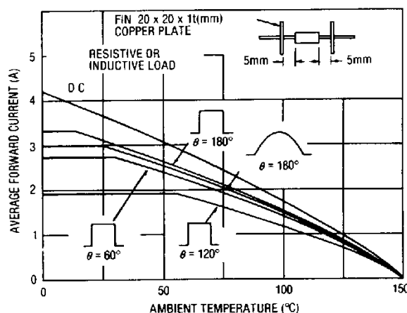
Fig. 19 — Average Forward Current Vs. Ambient Temperature
