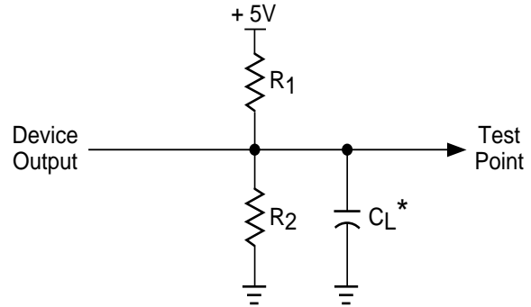
Figure 3. Test Load
