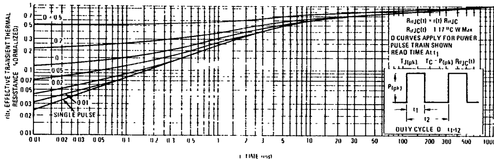
FIGURE 15 - THERMAL RESPONSE
