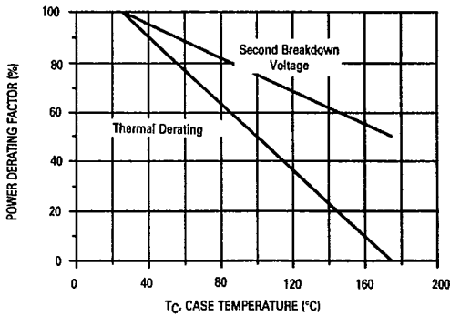
FIGURE 14 — POWER DERATING
