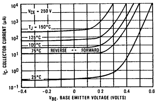
FIGURE 5 - COLLECTOR CUTOFF REGION
