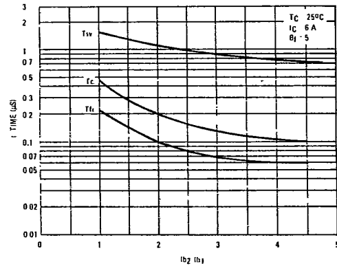
FIGURE 11b - TURN-OFF TIMES vs I_{B2}/I_{B1}
