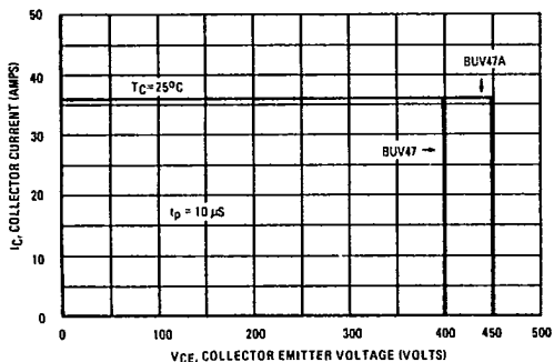
FIGURE 16 - RATED OVERLOAD SAFE OPERATING AREA (OLSOA)
