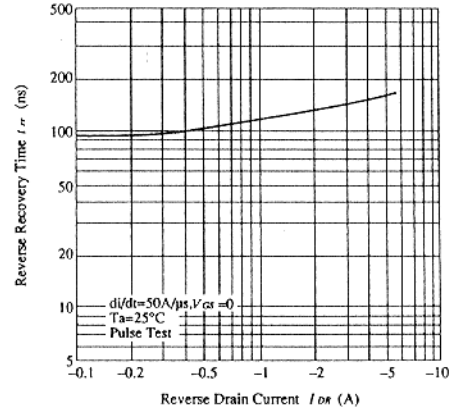
BODY-DRAIN DIODE REVERSE RECOVERY TIME
