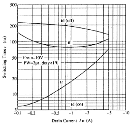
SWITCHING CHARACTERISTICS
