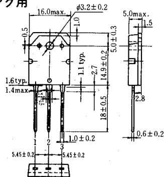
(TO-3P)
