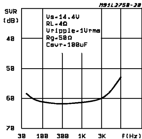
Figure 24: Supply Voltage Rejection vs. Frequency
