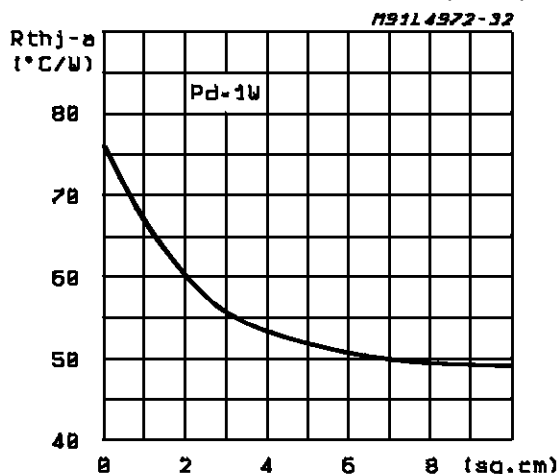
Figure 35: Junction to Ambient Thermal Resistance vs. Area on Board Heatsink (SO20)
