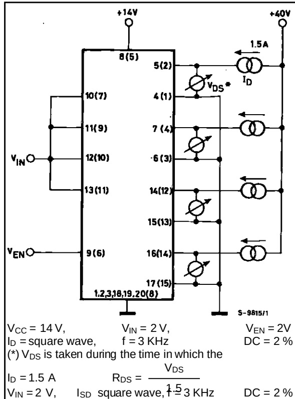
Figure 5 : R_{DS(on)} .
