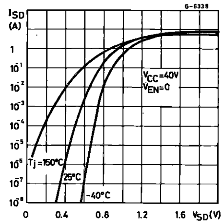
Figure 11 : Typical Source-drain Diode Forward Voltage.
