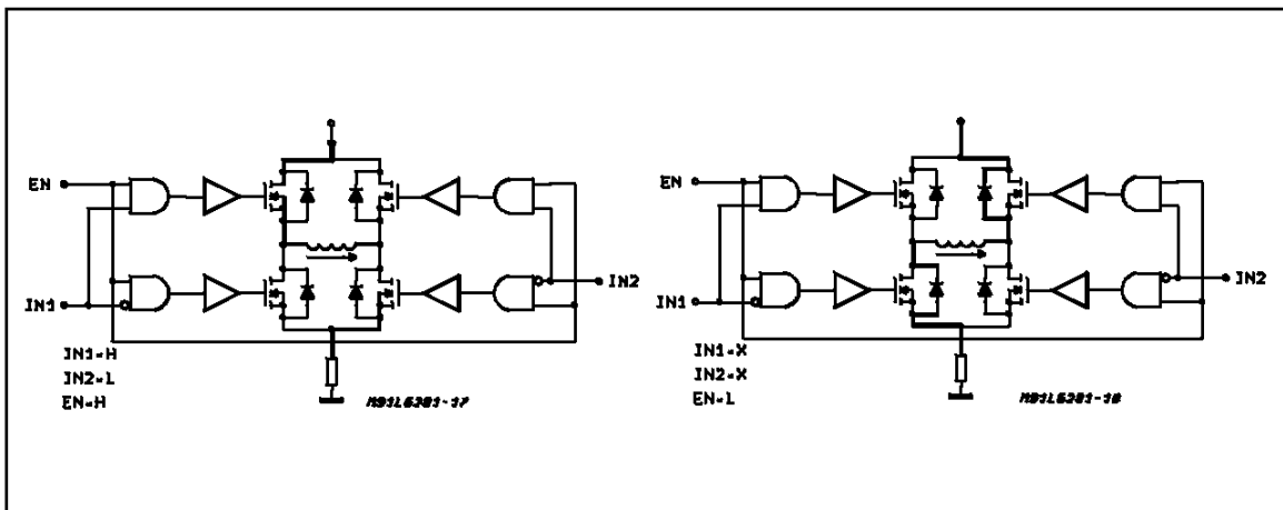
Figure 8c: Enable Chopping
