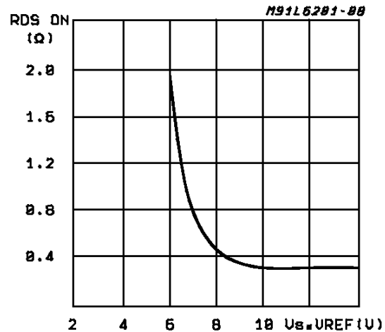
Figure 4: Typical R_{DS(ON)} vs. V_S \sim V_{REF}
