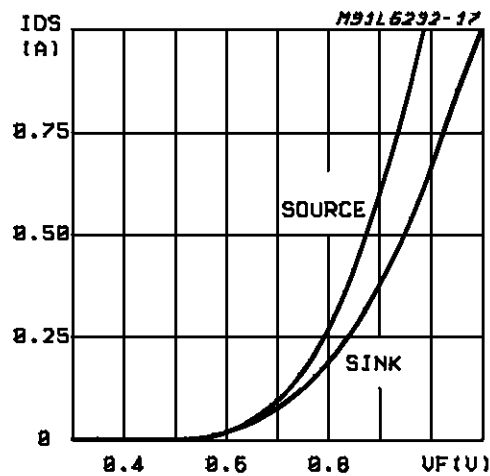
Figure 6: Typical Body Diode Forward Drop vs. Drain to Source Current.
