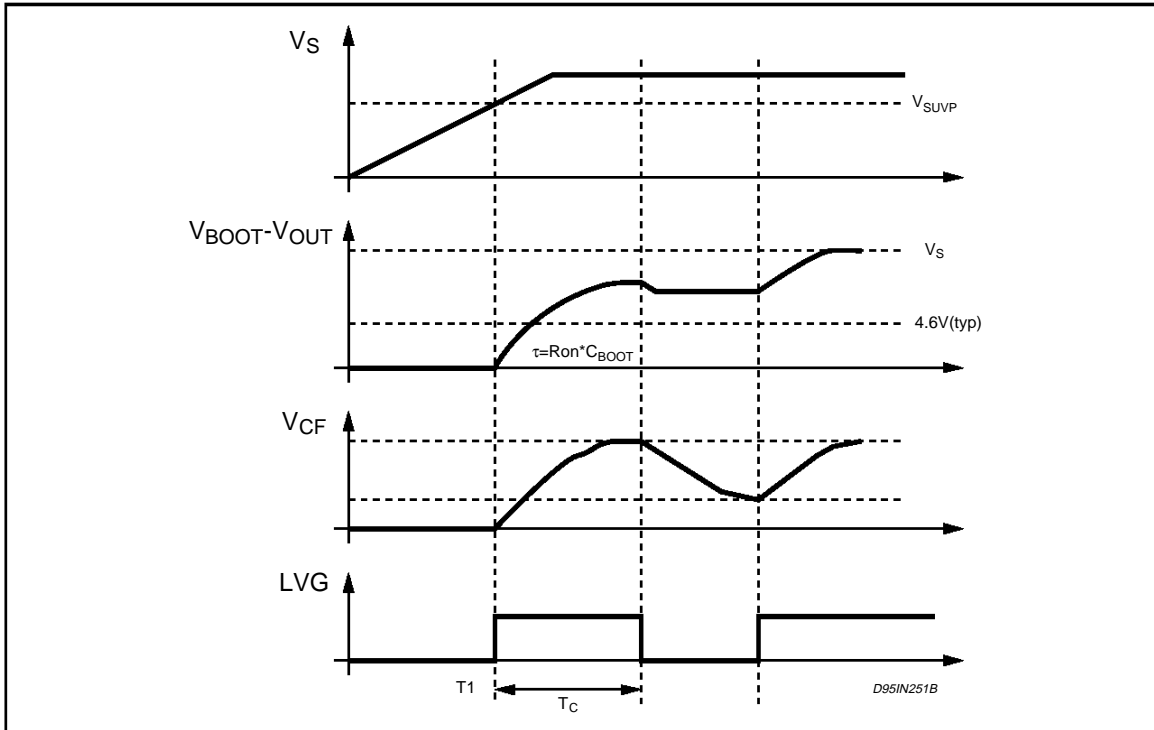
Figure 2: WAVEFORMS (L6569A)
