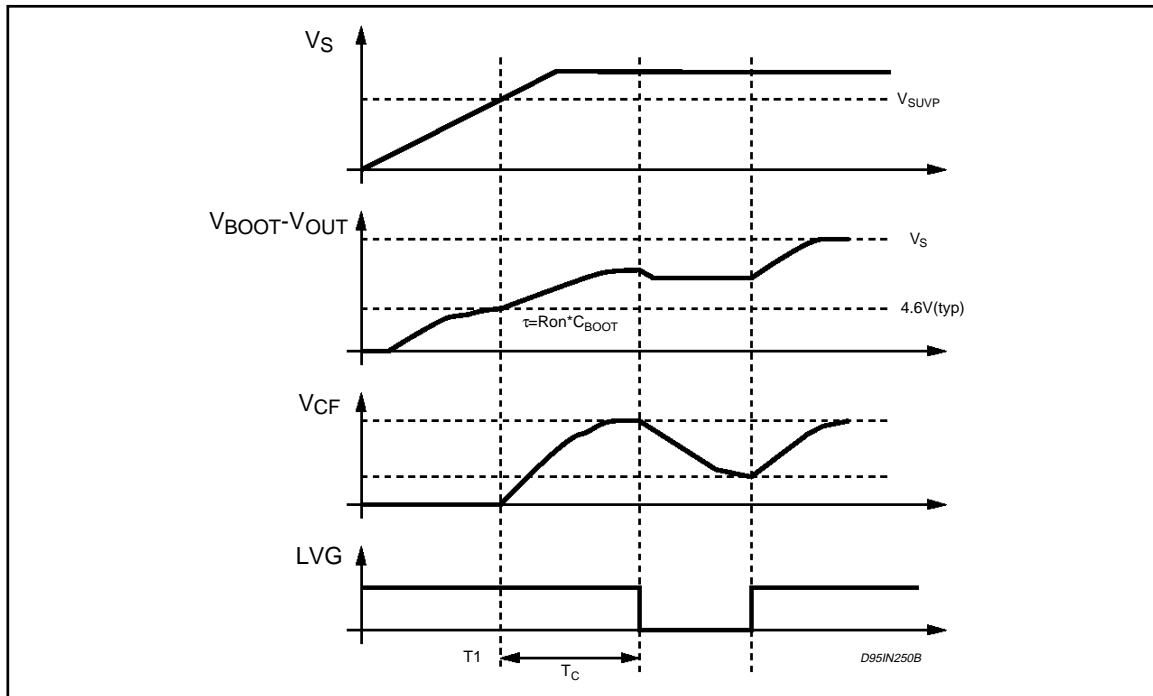
Figure 1: WAVEFORMS (L6569)
