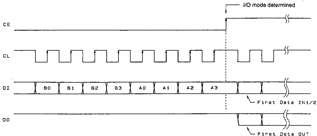
Figure 6 Mode Selection Address Bits
