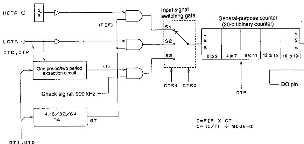
Figure 8 General-Purpose Counter
