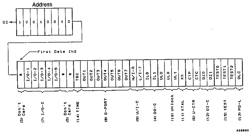
Figure 2 Input Data Word IN2
