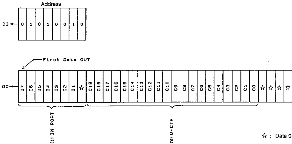
Figure 5 Output Data Word Out
