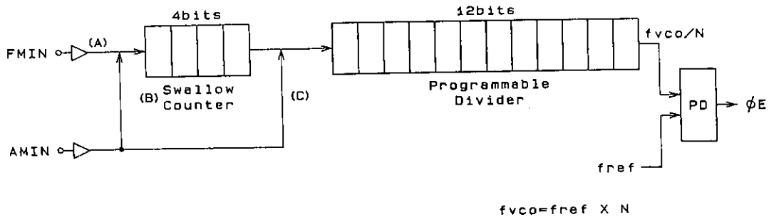
Figure 7 Programmable Divider
