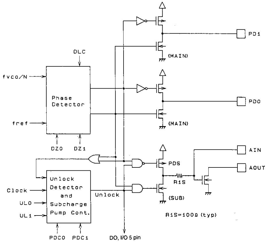
Figure 9 Charge Pump
