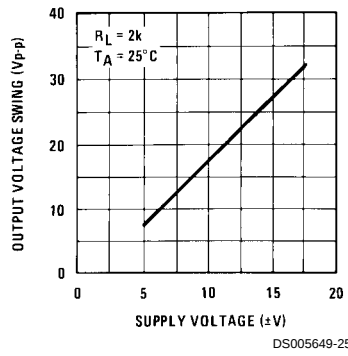
Voltage Swing
