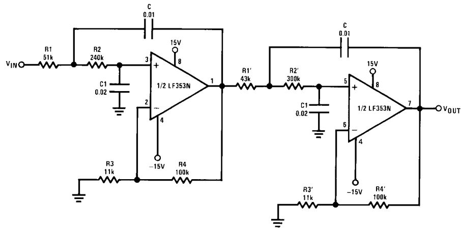
Fourth Order Low Pass Butterworth Filter
