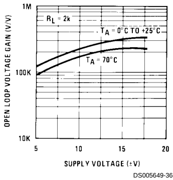
Open Loop Voltage Gain (V/V)
