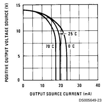
Positive Current Limit
