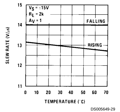
Slew Rate
