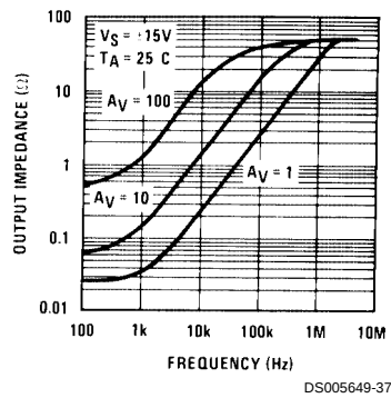
Output Impedance
