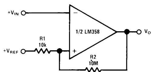
Comparator with Hysteresis
