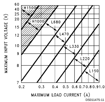
FIGURE 4. LM2575(HV)-5.0
