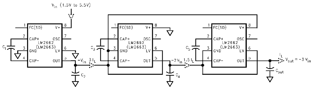
FIGURE 6. Generating -3V_{in} from +V_{in}
