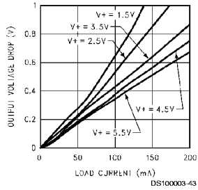
Output Voltage Drop vs Load Current
