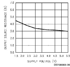
Output Source Resistance vs Supply Voltage
