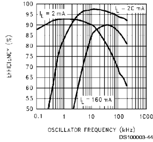
Efficiency vs Oscillator Frequency
