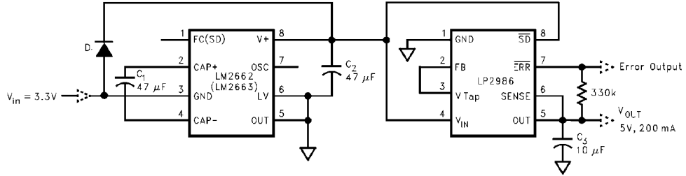
FIGURE 9. Generating +5V from +3.3V Input Voltage
