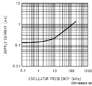
Supply Current vs Oscillator Frequency
