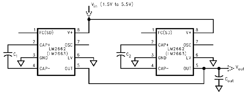
FIGURE 4. Lowering Output Resistance by Paralleling Devices
