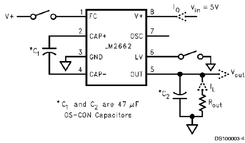
FIGURE 1. LM2662 and LM2663 Test Circuits
