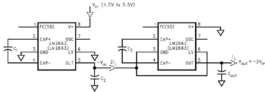
FIGURE 5. Increasing Output Voltage by Cascading Devices
