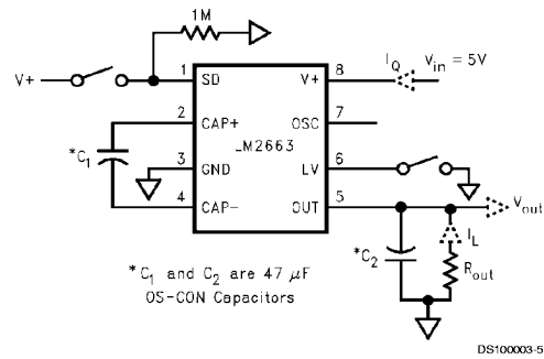
FIGURE 1. LM2662 and LM2663 Test Circuits
