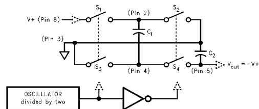
FIGURE 2. Voltage Inverting Principle
