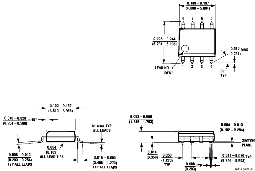
8-Lead SO (M) Order Number LM2662M or LM2663M NS Package Number M08A
