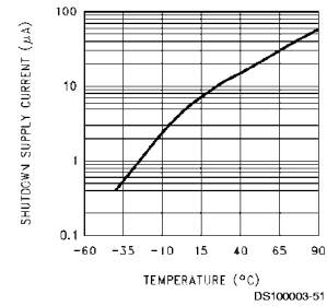
Shutdown Supply Current vs Temperature (LM2663 Only)
