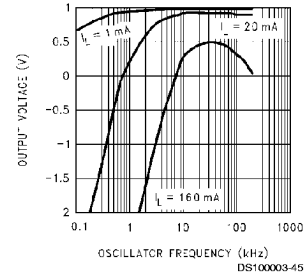
Output Voltage vs Oscillator Frequency
