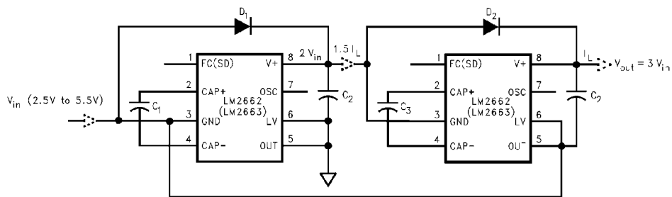
FIGURE 7. Generating +3V_{in} from +V_{in}
