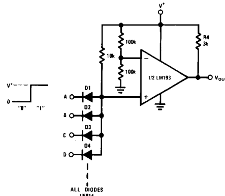
Large Fan-in AND Gate
