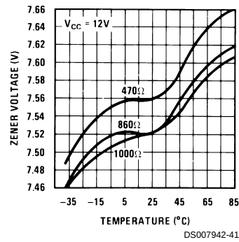
Zener Voltage vs Temperature
