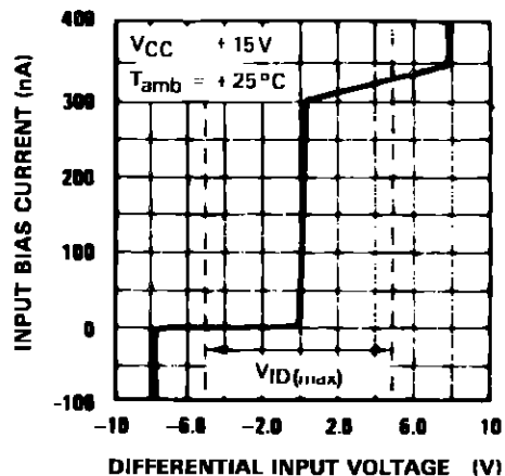
INPUT CHARACTERISTICS
