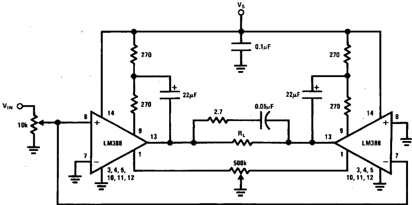
FIGURE 4. Amplifier with Gain = 200 and Minimum C_B
