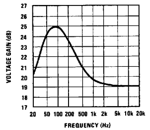
FIGURE 6b. Frequency Response with Bass Boost
