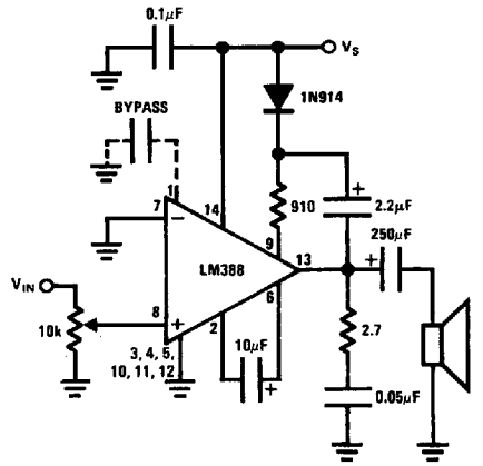
FIGURE 4. Amplifier with Gain = 200 and Minimum C_B
