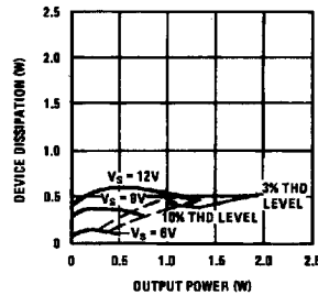
Device Dissipation vs Output Power—16 Ohm Load
