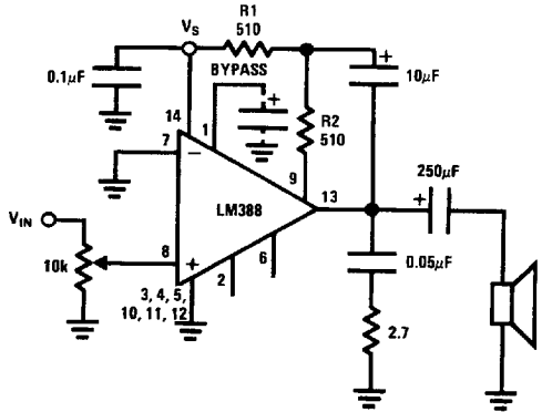
FIGURE 1. Load Returned to Ground (Amplifier with Gain = 20)
