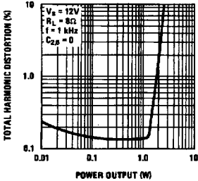
Distortion vs Output Power
