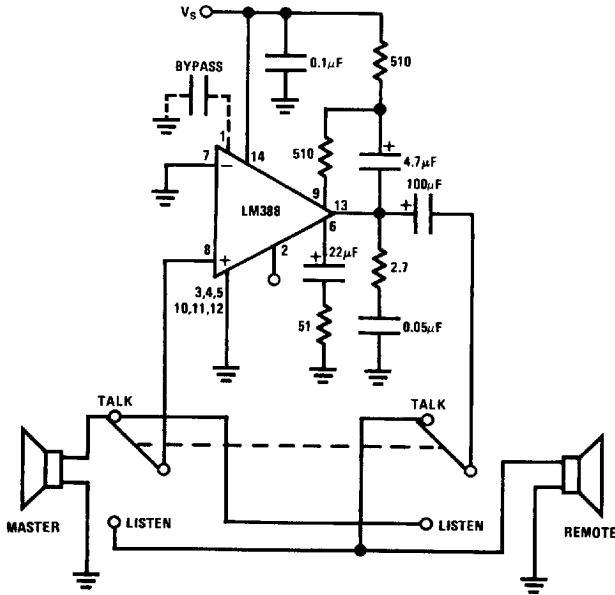
FIGURE 7. Intercom
