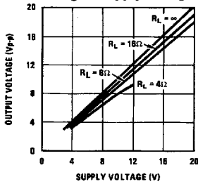
Peak-to-Peak Output Voltage Swing vs Supply Voltage
