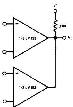
ORing the Outputs
