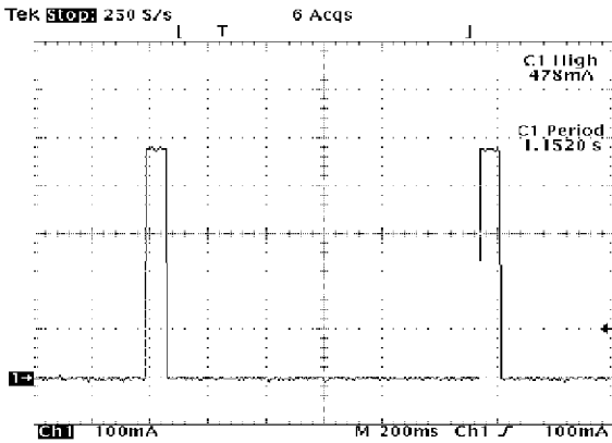
Dynamic Overload protection (Isc vs Time)
