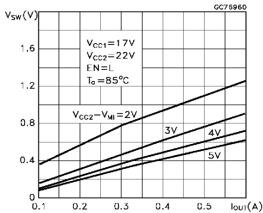
Bypass Switch Drop vs Output Current
