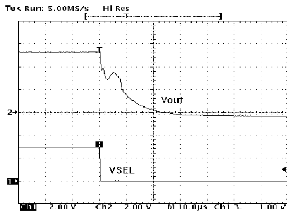
18V to 13V Change
