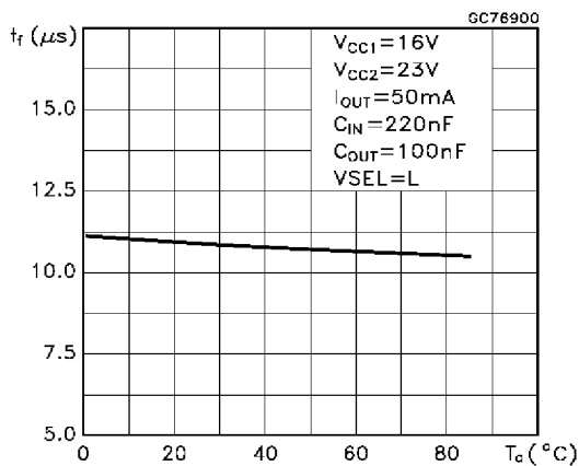
Tone Fall Time vs Temperature
