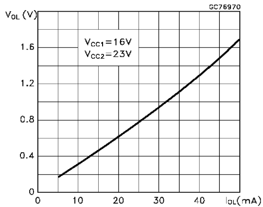
Overload Flag pin Logic Low vs Flag Current
