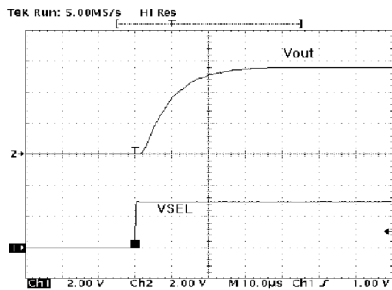
13V to 18V Change
