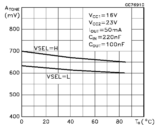
Tone Amplitude vs Temperature
