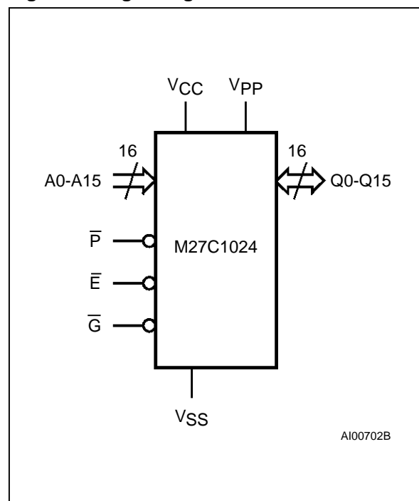
Figure 1. Logic Diagram
