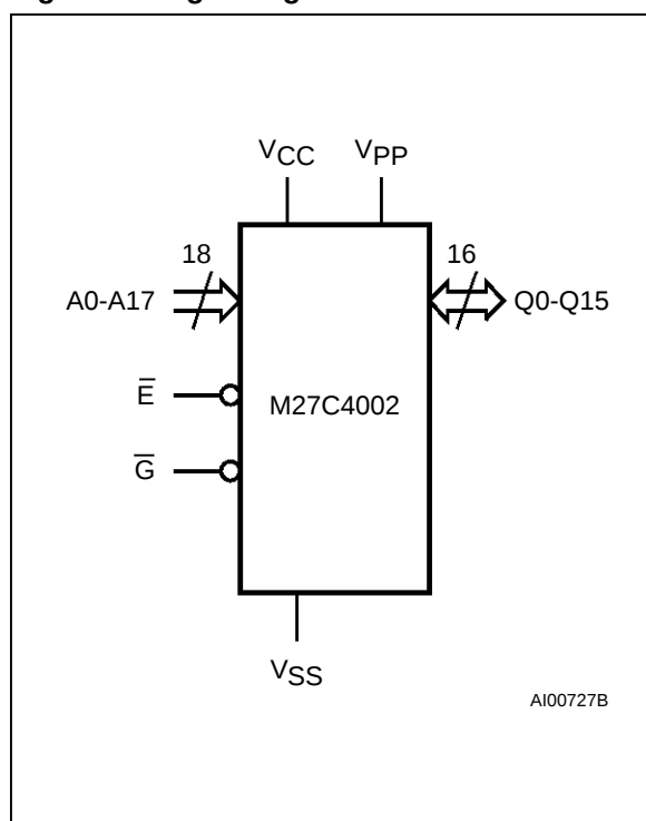
Figure 1. Logic Diagram
