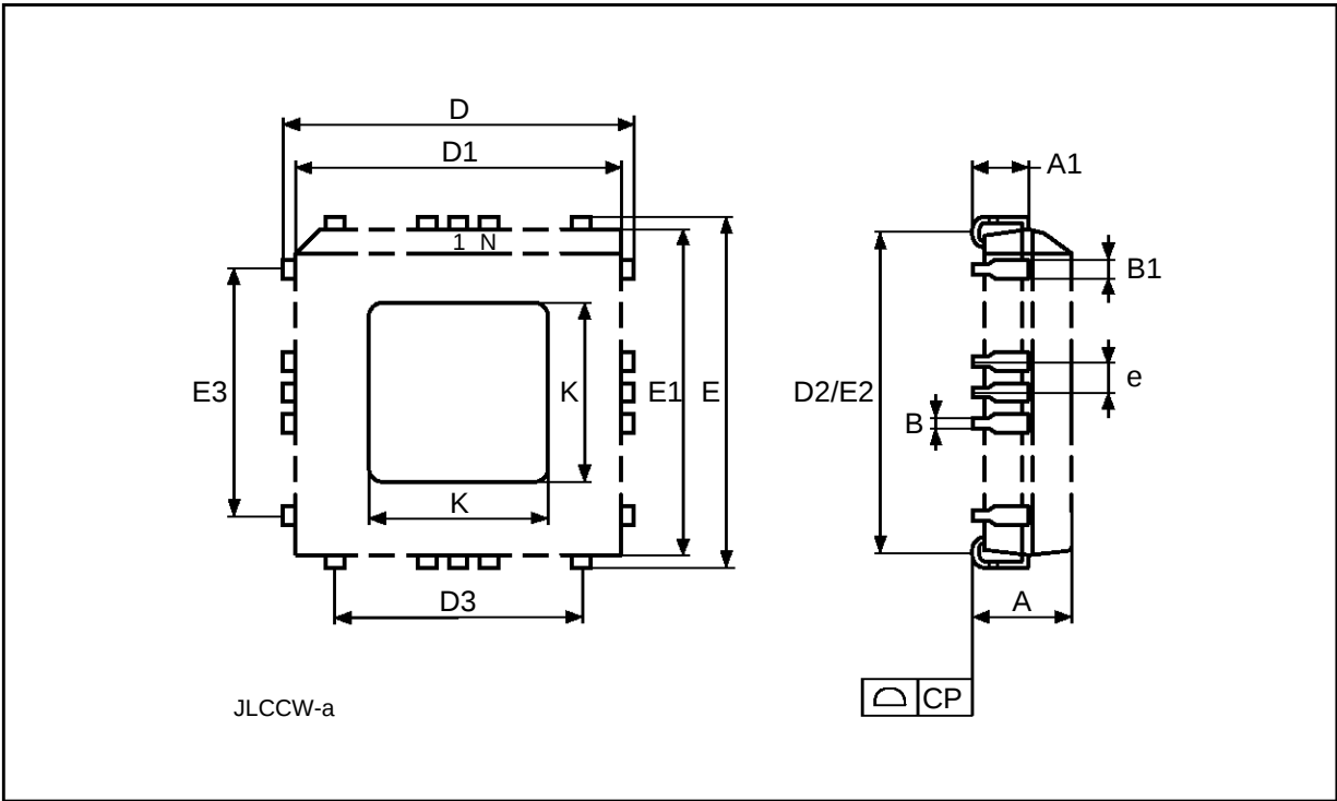
JLCC44W
