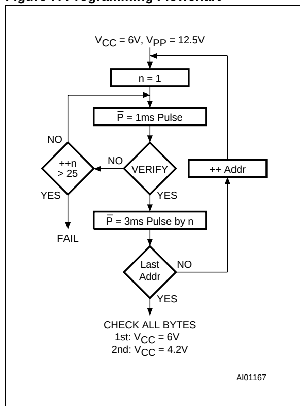
Figure 7. Programming Flowchart
