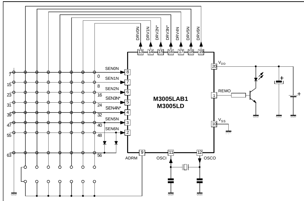
Figure 1 : Typical Application
