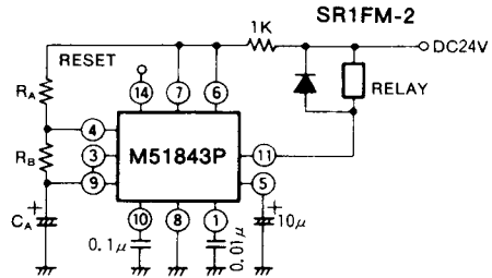
(2) ASTABLE OPERATION
