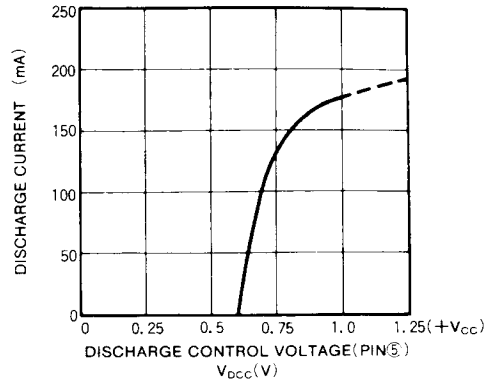
DISCHARGE CONTROL CHARACTERISTICS
