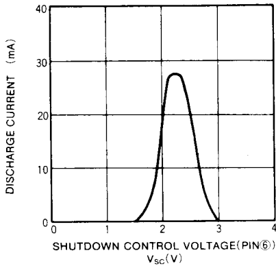
SHUTDOWN CONTROL CHARACTERISTICS
