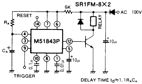
(1) DELAY TIMER
