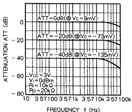
ATTENUATION VS. FREQUENCY
