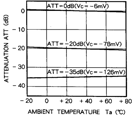
ATTENUATION VS. AMBIENT TEMPERATURE (TEMPERATURE COMPENSATION)
