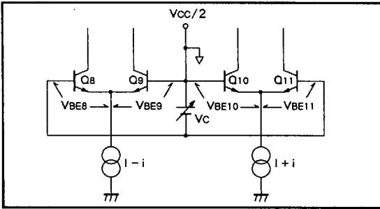
Fig. 2 Differential circuit
