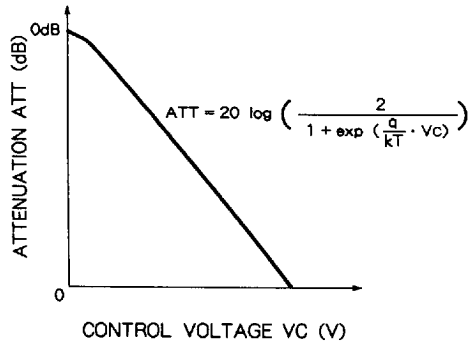
ATTENUATION VS. CONTROL VOLTAGE
