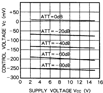
CONTROL VOLTAGE VS. SUPPLY VOLTAGE
