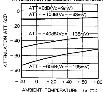
ATTENUATION VS. AMBIENT TEMPERATURE
