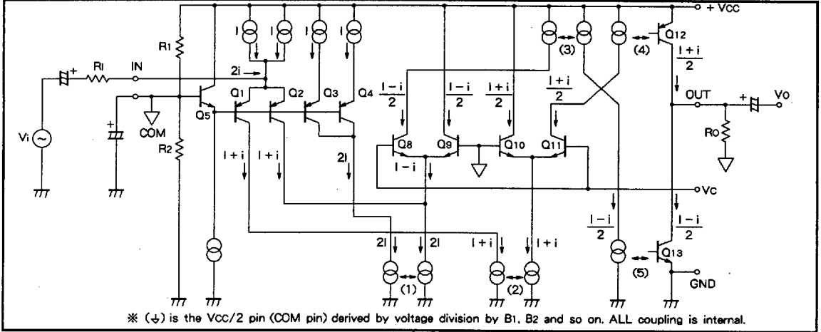
Fig. 1 M5222 Equivalent circuit
