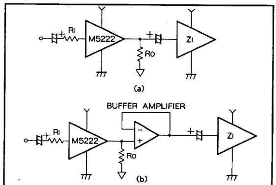
Fig. 5 Connection example
