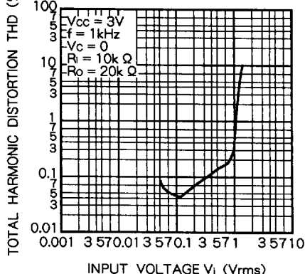
TOTAL HARMONIC DISTORTION VS. INPUT VOLTAGE
