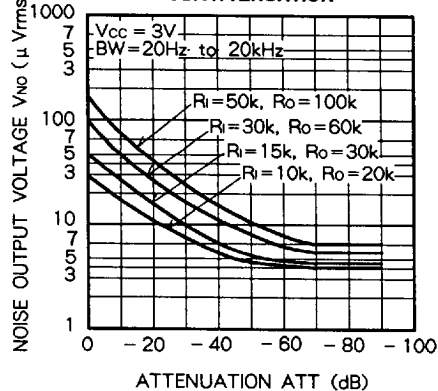
NOISE OUTPUT VOLTAGE VS. ATTENUATION
