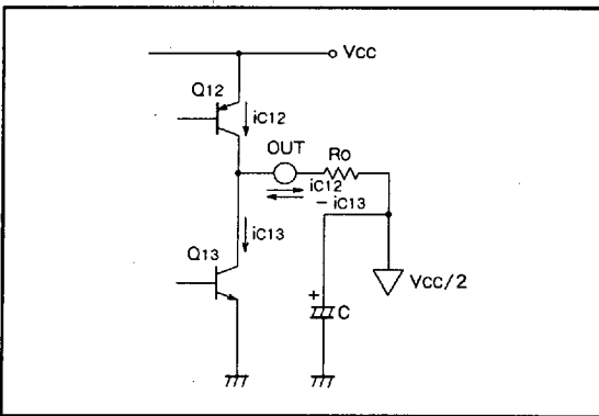
Fig. 4 Equivalent circuit of output stage
