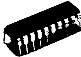
Outline 20P4(P) 2.54mm pitch 300mil DIP (6.3mm x 24.0mm x 3.3mm)
