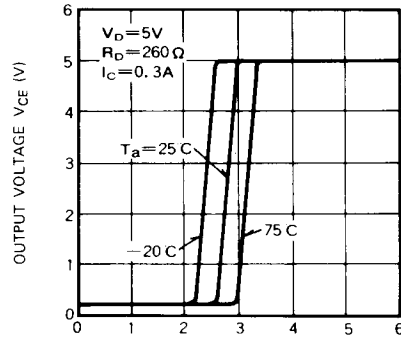
INPUT VOLTAGE V_i (V)
