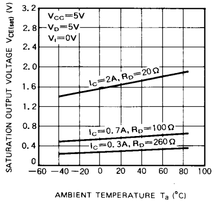
SATURATION OUTPUT VOLTAGE VS. AMBIENT TEMPERATURE
