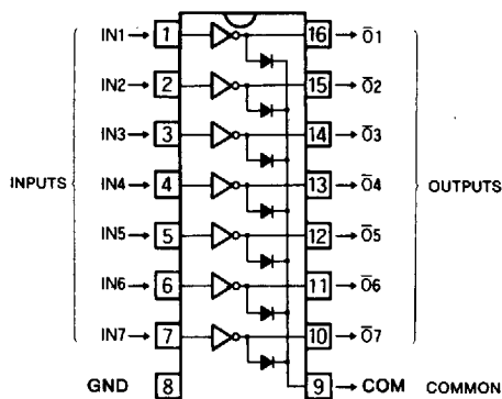
Outline 16P4
