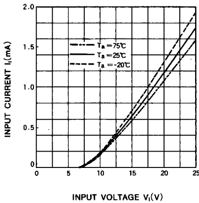
INPUT CHARACTERISTICS
