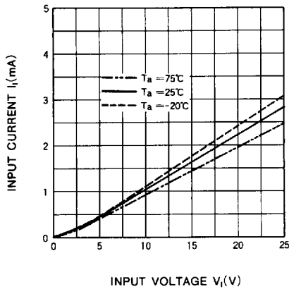
INPUT CHARACTERISTICS
