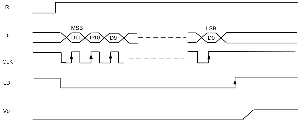
TIMING CHART (MODEL)
