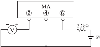
Fig1. Measurement Circuit
