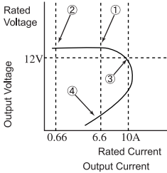
Fig2. Output Voltage/Current
