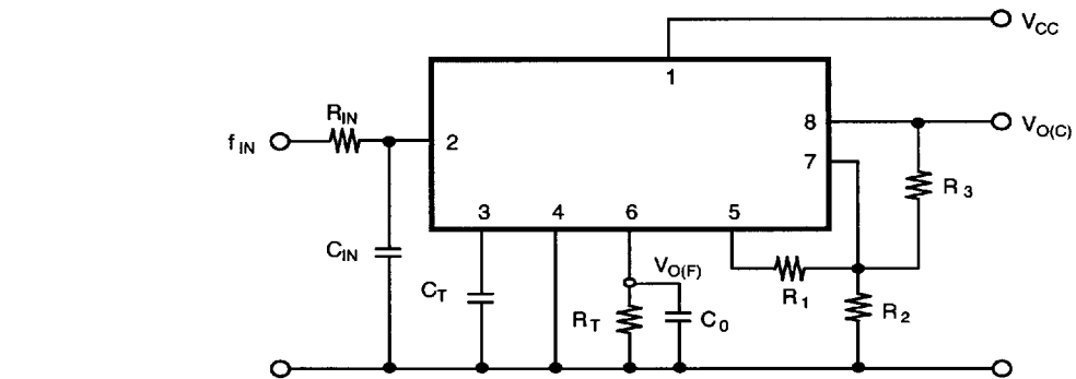
FIG. 2 — TYPICAL HOOKUP AND OPERATING PARAMETERS
