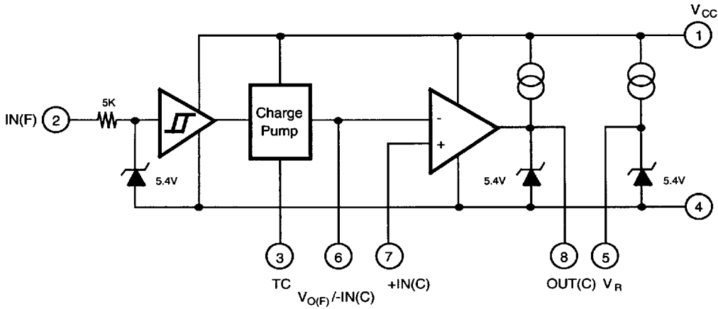
Fig. 1 — MB4206 BLOCK DIAGRAM
