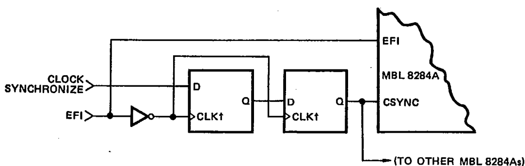
Fig. 3 – CSYNC SYNCHRONIZATION
