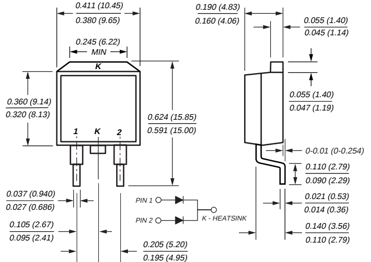
TO-263AB (MBRB15xxCT)
