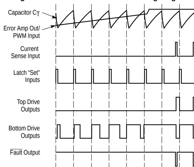
Figure 21. Pulse Width Modulator Timing Diagram
