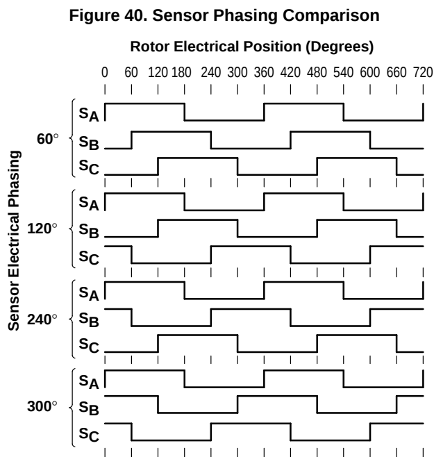
Figure 41. Sensor Phasing Table
