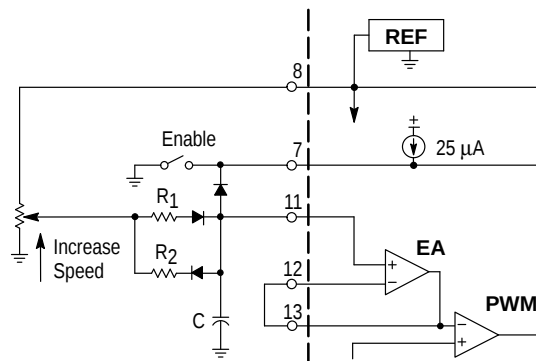
Figure 32. Controlled Acceleration/Deceleration
