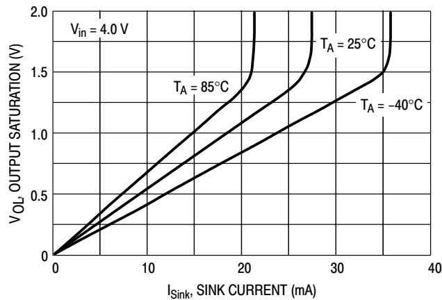
Figure 5. \overline{\text{Reset}} Output Saturation versus Sink Current
