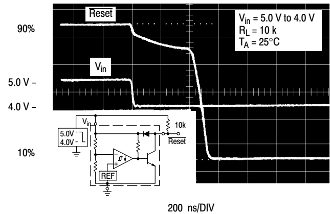
Figure 6. \overline{\text{Reset}} Delay Time
