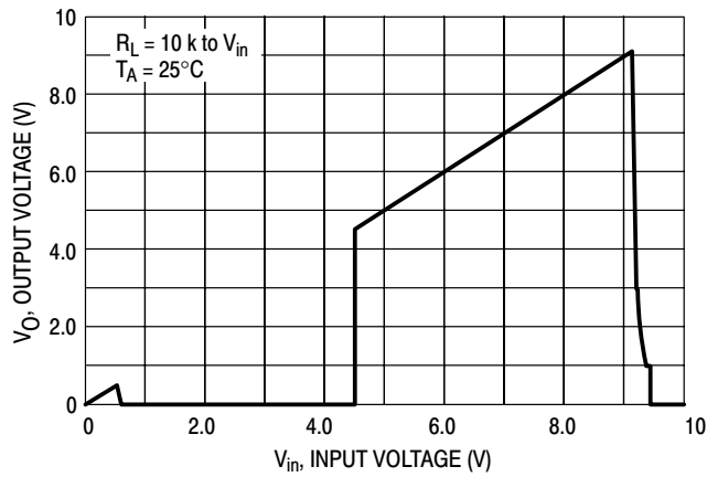
Figure 1. \overline{\text{Reset}} Output Voltage versus Input Voltage
