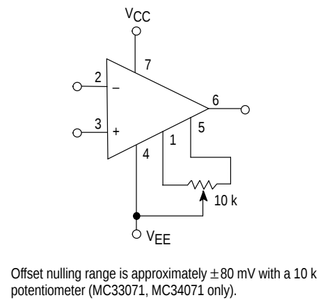
Figure 2. Offset Null Circuit
