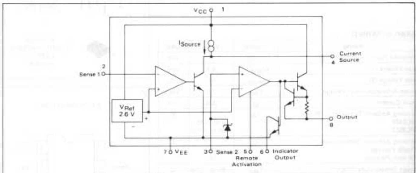
FIGURE 1 – BLOCK DIAGRAM
