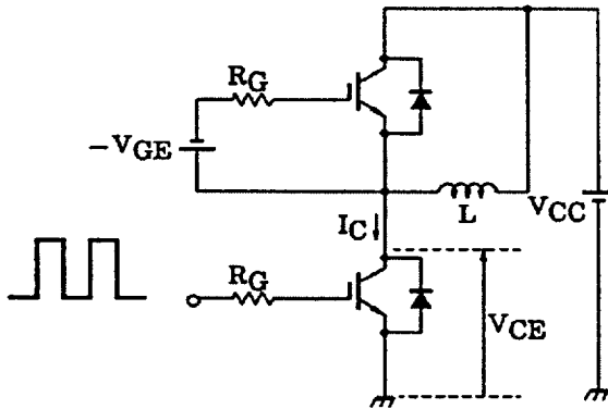
Note. 1 Switching Time Test Circuit & Timing Chart
