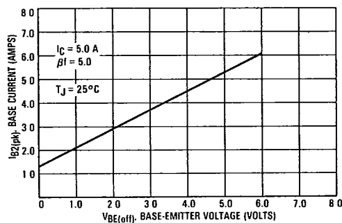
FIGURE 8 - PEAK REVERSE CURRENT
