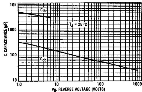
FIGURE 6 — CAPACITANCE
