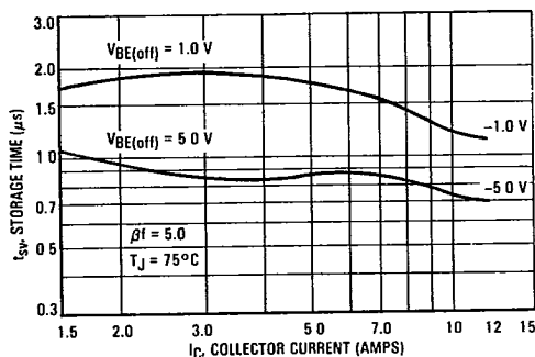
FIGURE 9 — STORAGE TIME
