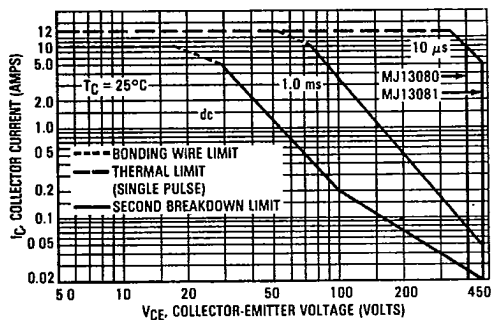
FIGURE 12 — FORWARD BIAS SAFE OPERATING AREA
