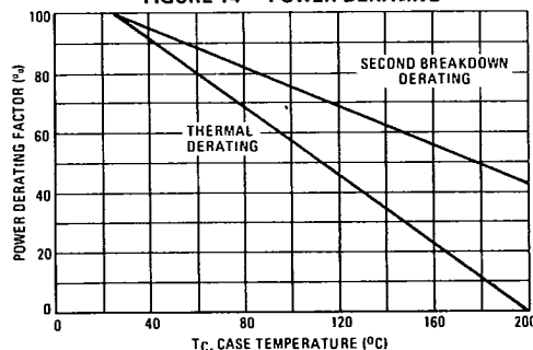
FIGURE 14 — POWER DERATING
